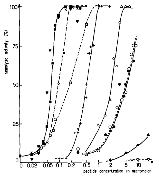
Fig. 4. Hemolysis induced by the amphipathic peptides on 10^7 cells/ml at 37°C, Tris buffer 20 mM, 130 mM NaCl, pH 7.5. Natural cytotoxins: (+) Mel; (▲) Magainin; (▽) Mastoparan. Synthetic dansylated peptides of increasing length: (○) 12-; (×) 15-; (●) 18-; (△) 19-; (▼) 20-; (□) 21-; (■) 22-mers.
